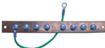
Ground bar for Floor mount cabinet
